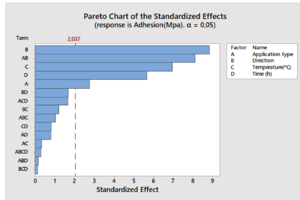
Figure 1. Pareto chart for the effective factors
