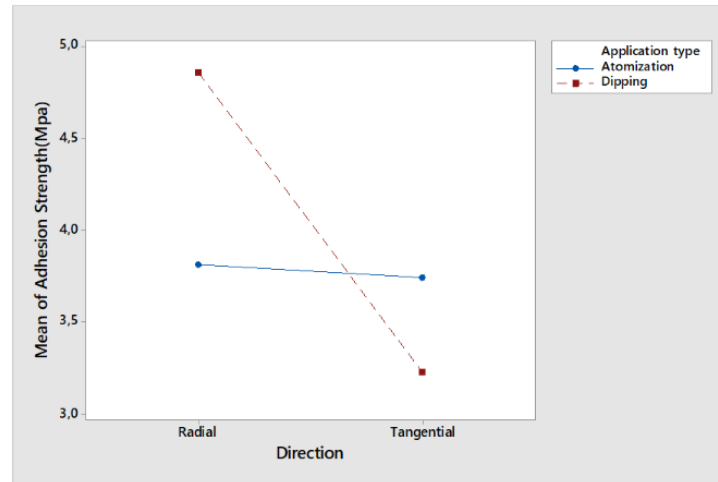
Figure 3. Interaction between application type and direction
