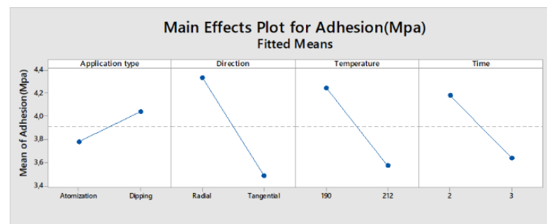
Figure 2. Main effect plot of adhesion strength
