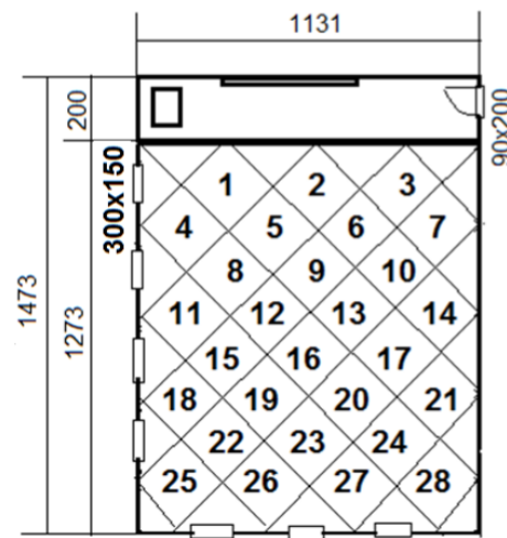
Figure 5. Cross-row classroom plan (cm)
