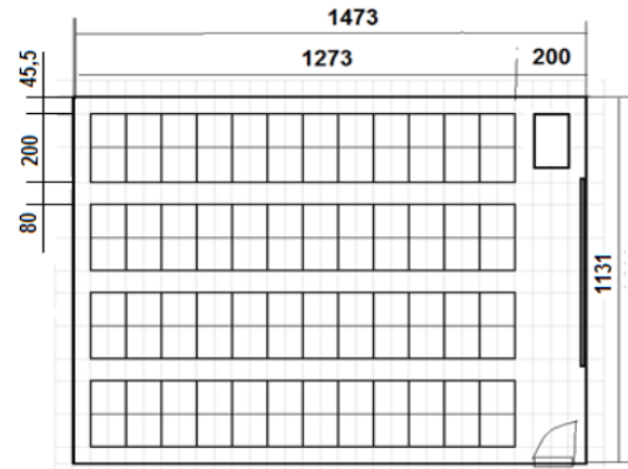
Figure 8. Straight row classroom design for normal conditions
