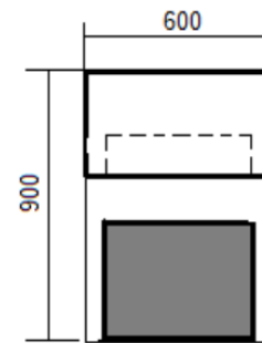
Figure 2. Student desk and seat; top view / projection
