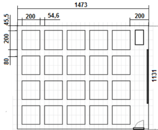
Figure 7. Flat-row classroom design for COVID-19 conditions
