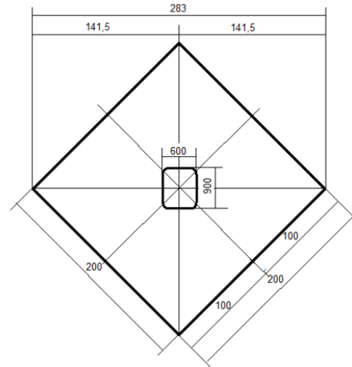
Figure 4. Diagonal placement cell (cm)
