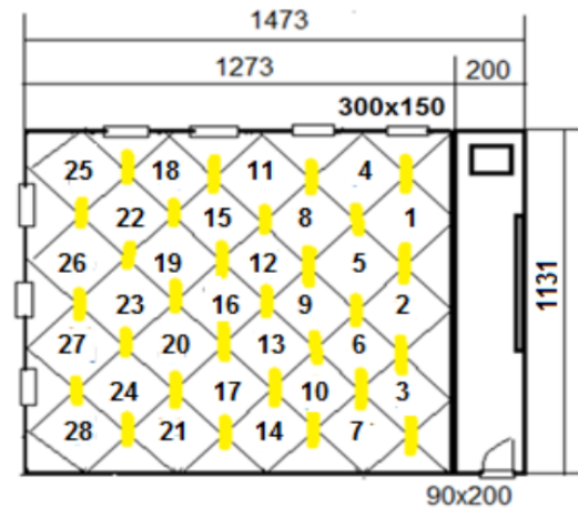
Figure 9. Cross-row classroom artificial lighting arrangement (cm)
