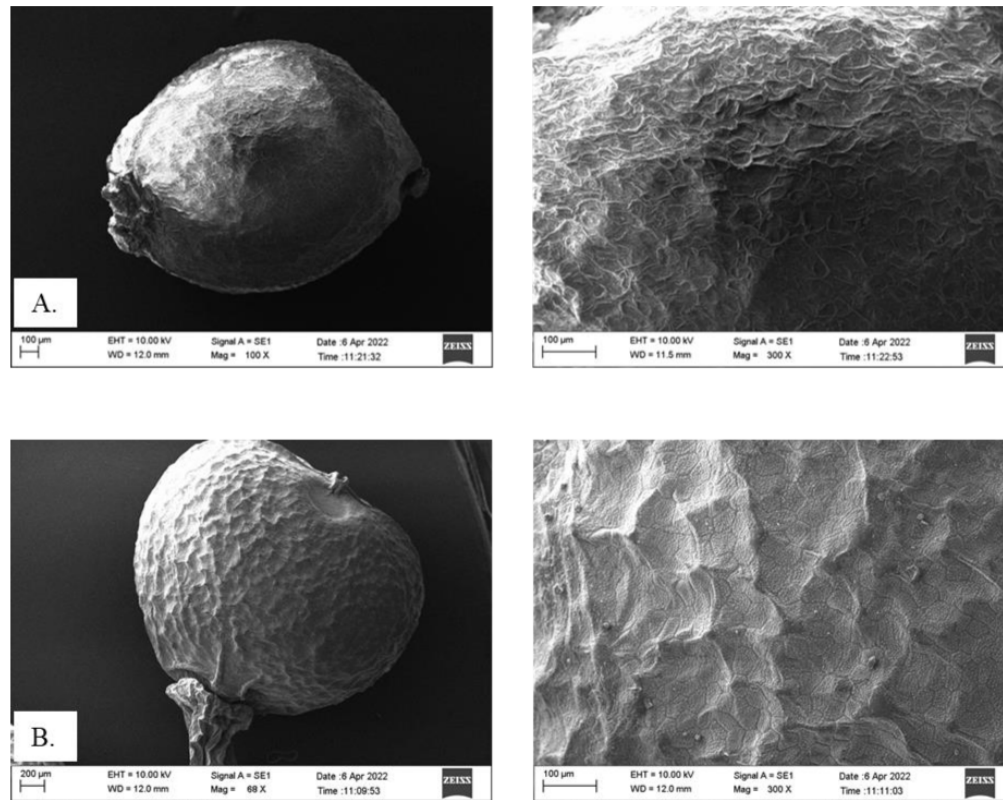
Figure 2. SEM images of fruit (A) F. asepalae (B) F. schleicheri subsp. microcarpa
