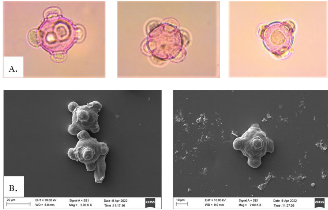
Figure 5. F. asepalae pollen (A-Light microscope images B-SEM images)
