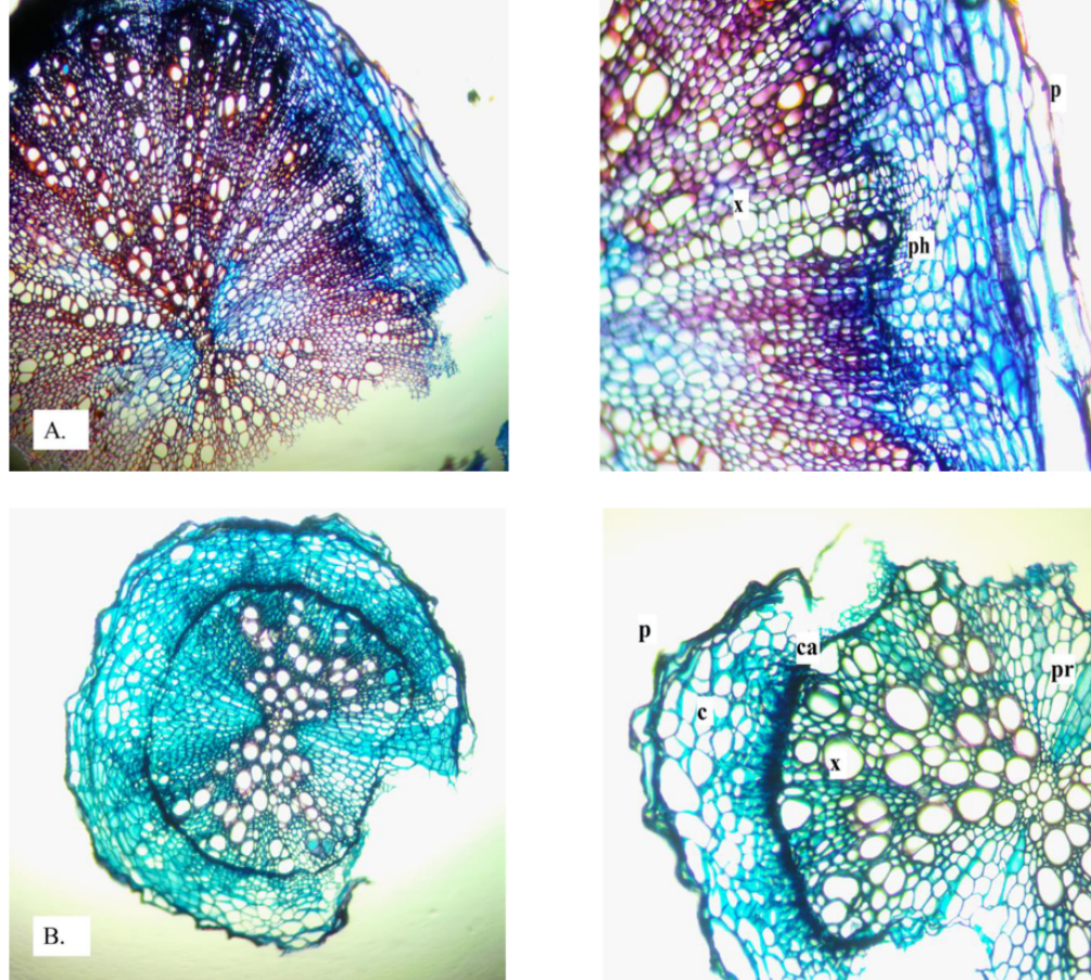
Figure 3. Photomicrographs of root (A) F. asepala (B) F. schleicheri subsp. microcarpa (p-peridermis, c-korteks, ca-cambiyum, x-xylem, pr-pith ray, ph-phloem)
