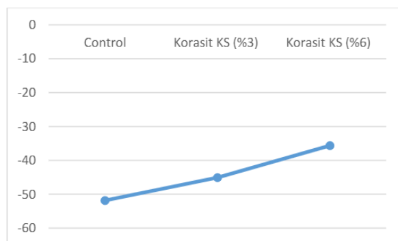
Figure 3. Gloss test values after weathering (%)
