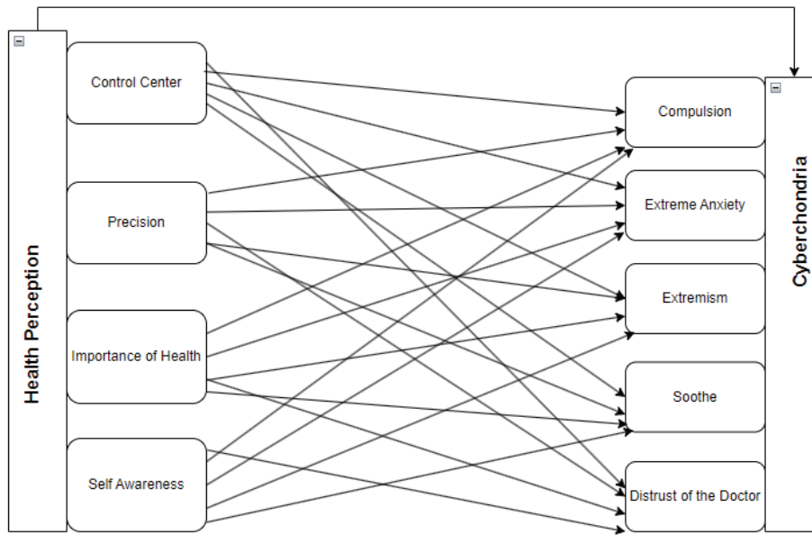
Figure 1: Research model
