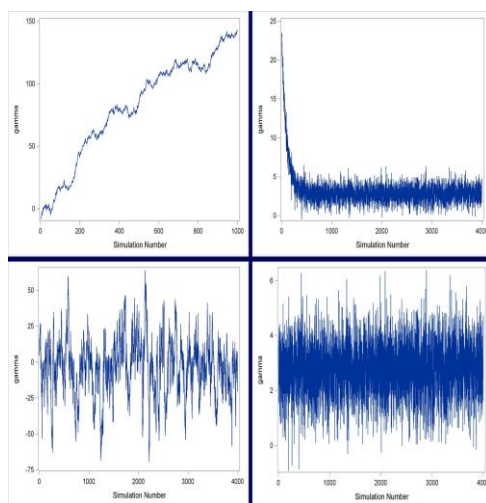
Figure 1 Some typical features that can be seen in the trace graph
