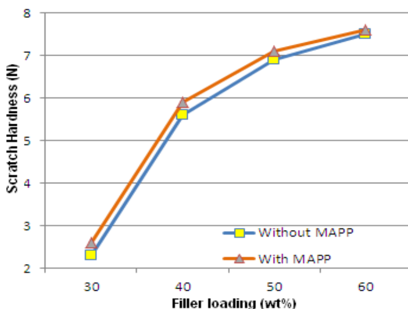
Fig. 3. Effects of WSF content and coupling agent (MAPP) on the scratch hardness of the PP composite (WSF: waste sunflower stalk flour)
