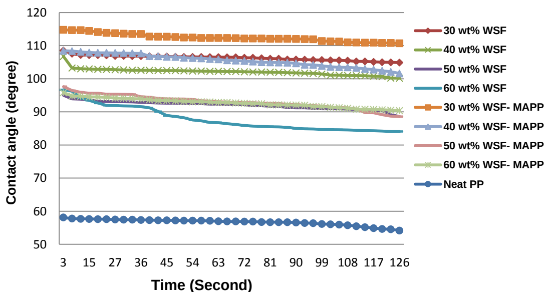
Fig. 2. Effects of WSF content and coupling agent (MAPP) on the contact angle of the PP composite (WSF: waste sunflower stalk flour)
