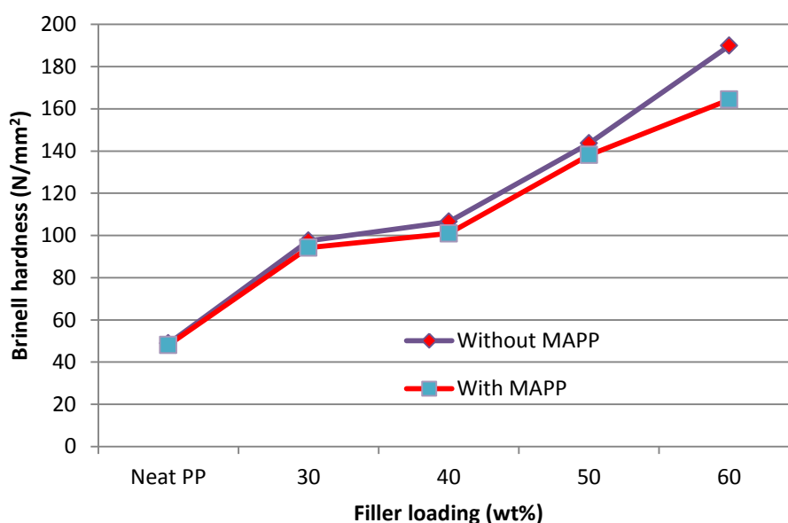
Fig. 4. Effects of WSF content and coupling agent (MAPP) on the Brinell hardness of the PP composite (WSF: waste sunflower stalk flour)
