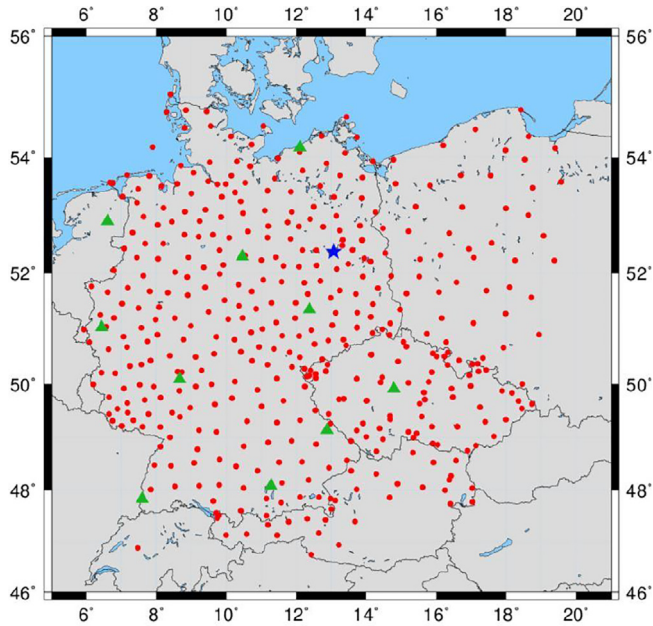
Fig. 1. GNSS stations located in central Europe covering Germany and large parts of Poland, Czech Republic and Austria. Blue star represents station POTS, green triangles denote the stations utilized in the case study. In total, there are 431 stations.
