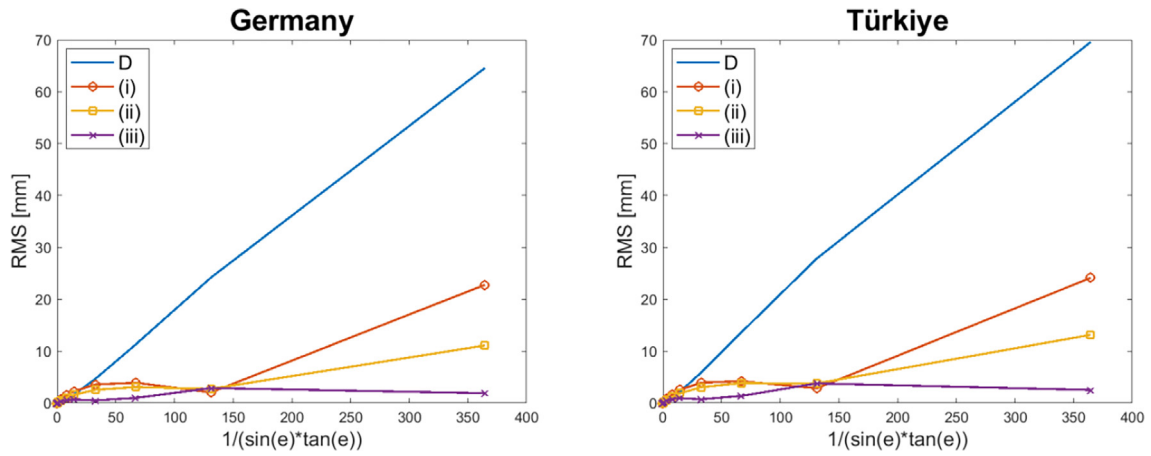
Fig. 3. RMS deviation as a special function of the elevation angle for the approaches. The left plot shows the result for Germany the right plot shows the result for Türkiye. For details the reader is referred to the text.
