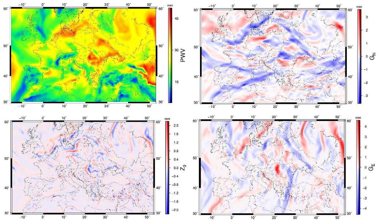
Fig. 4. The regional PWV, G_N , G_E and the additional parameter Z_0 that is used to modify the wet MF for July 1, 2021 07 UTC (first approach).
