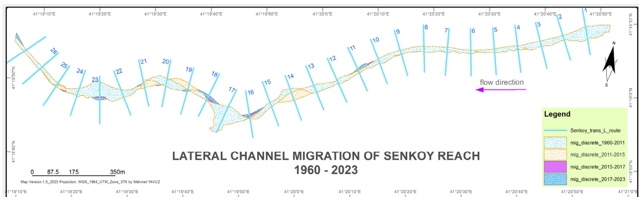
Figure 9. The lateral channel migration from 1960 to 2023 in Senkoy Reach within the Arhavi River Watershed (Türkiye). The shaded areas represent the discrete migration region from 1960 to 2011 (light blue), 2015 (orange), 2017 (magenta), and 2023 (blue) stream channel centerlines. The cross-section ID numbers increase along the flow direction.
