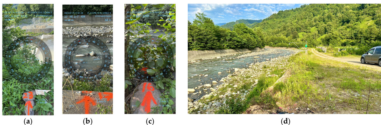
Figure 10. The cross-section transect conditions during the field measurements (a) transect 23 with partial vegetation cover, (b) an open cross-section transect 17 with no obstruction and the concrete confinement walls can easily be seen, (c) the cross-section transect 16 with heavy vegetation obstruction, and (d) a part of Sidere Creek and its floodplain on the right. The alluvial bars can be seen within the streams. Photos were captured by Mehmet Yavuz during the field measurements.
