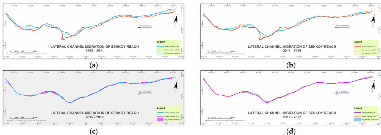
Figure 5. Maps of the reach-average channel migration rates of Senkoy Reach within the Arhavi River Watershed for the periods (a) 1960–2011, (b) 2011–2015, (c) 2015–2017, and (d) 2017–2023. The shaded areas show the lateral channel migrated polygons for each period.
