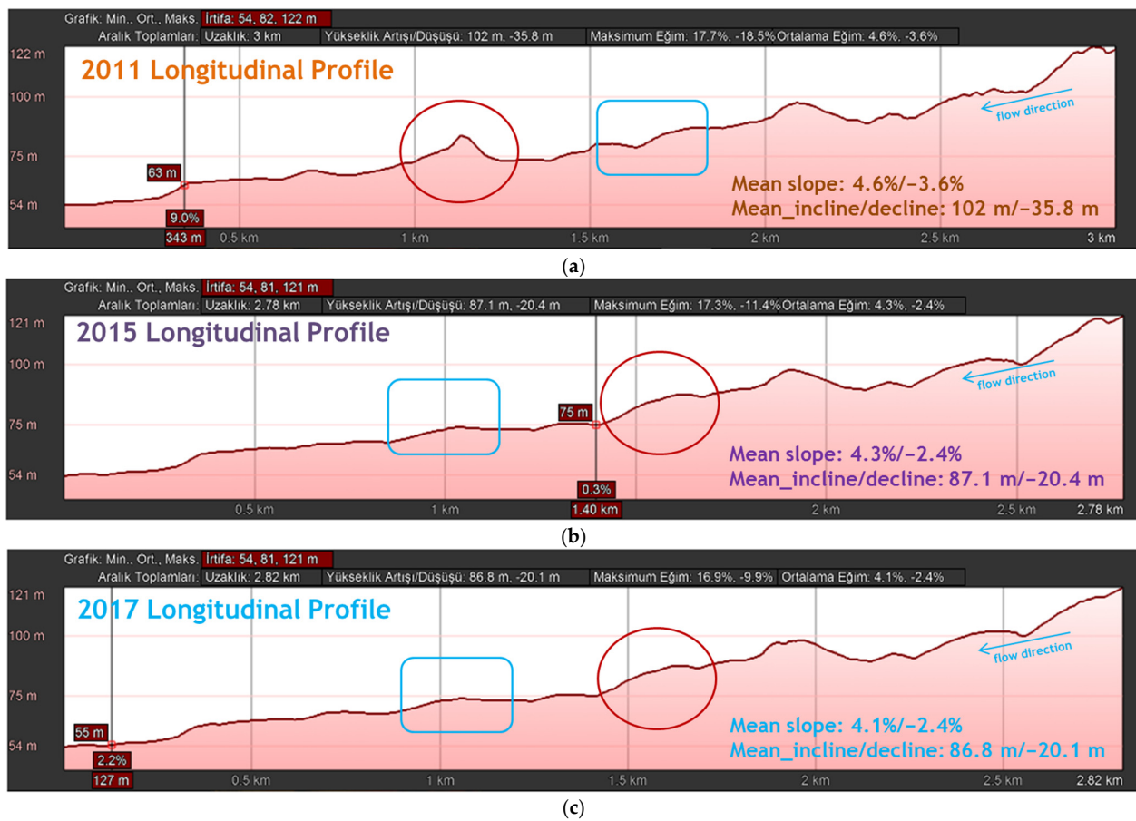
Figure 4. Longitudinal profiles of Senkoy Reach within the Arhavi River Watershed from (a) 2011, (b) 2015, and (c) 2017. The red circle indicates deposition and the blue rectangle indicates erosion on the stream bed.
