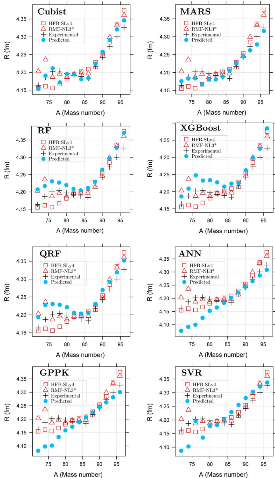
Figure 3. Predicted charge radius values for ^{72-96}\text{Kr} isotopes from Cubist, MARS, RF, XGBoost, QRF, ANN, GPPK, SVR models. The experimental data [5] and the predictions of HFB-SLy4 [108] and RMF-NL3* [109] are shown for comparison.
