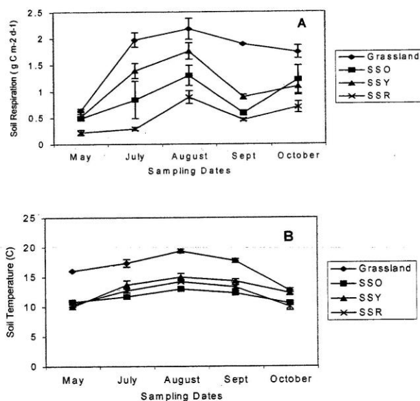
Figure 1: Mean monthly ( \pm 1 SE) soil respiration rates (A) and soil temperature (B) in young (SSY) and old oriental spruce stands with (SSR) / without understory (SSO) and in adjacent grasslands.
