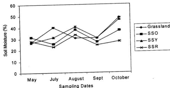
Figure 2: Mean monthly ( \pm 1 SE) soil moisture contents (0-5 cm depth) in young (SSY) and old oriental spruce stands with (SSR) / without understory (SSO) and in adjacent grasslands
