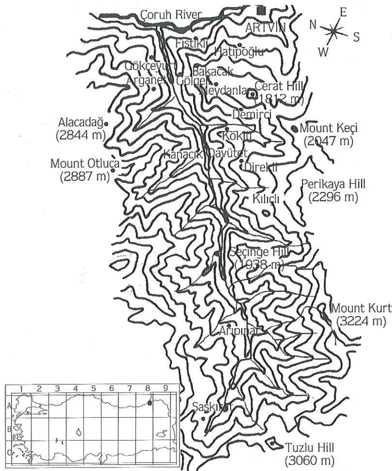
Figure 1. Topographical map of the study area.
