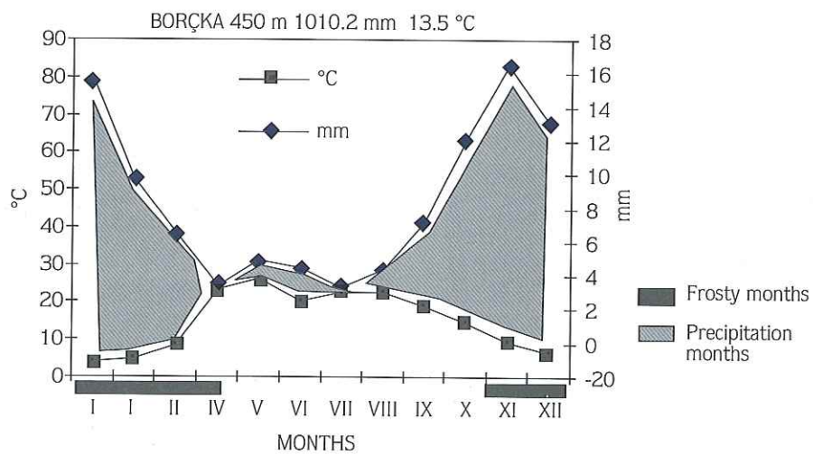
Figure 2. Climatic diagram of Borçka.
