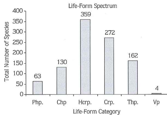
Figure 3. Life-form spectrum of the vascular flora of Camili.
