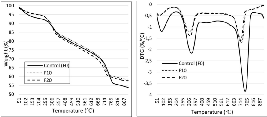
Figure 1: TGA/DTG curves of CBWPs containing FA.
