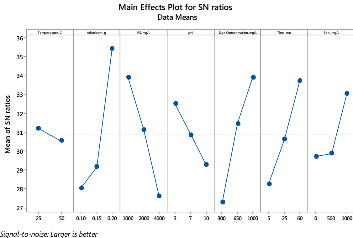
Fig. 5 S/N ratios of operating parameters on COD removal for HPS
