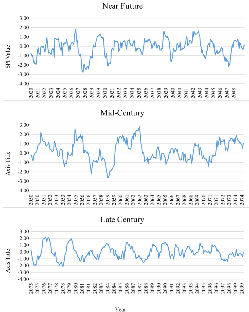
Fig. 3 SPI-12 index time series according to SSP2-4.5 scenario
