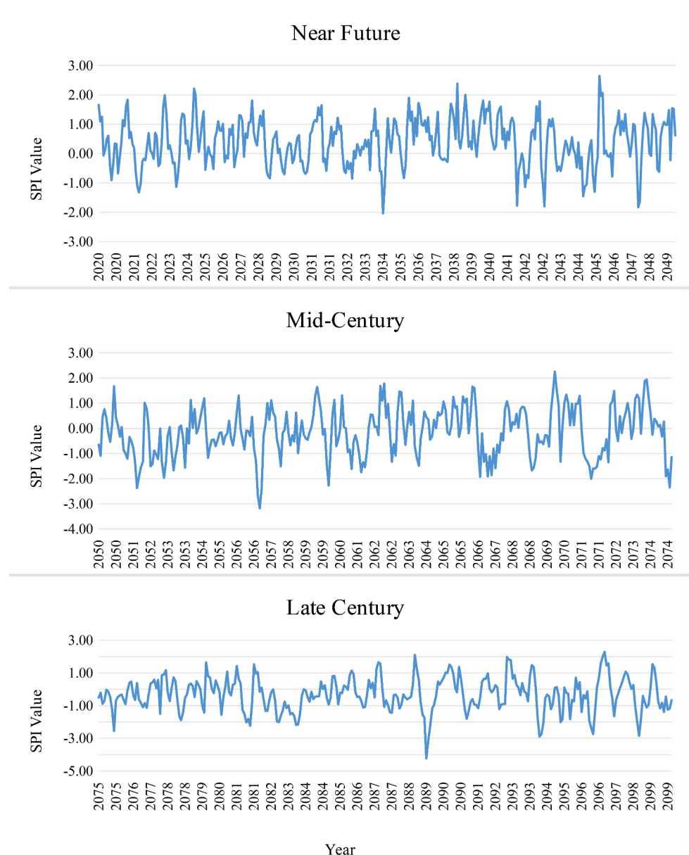
Fig. 4 SPI-3 index time series according to SSP5-8.5 scenario
