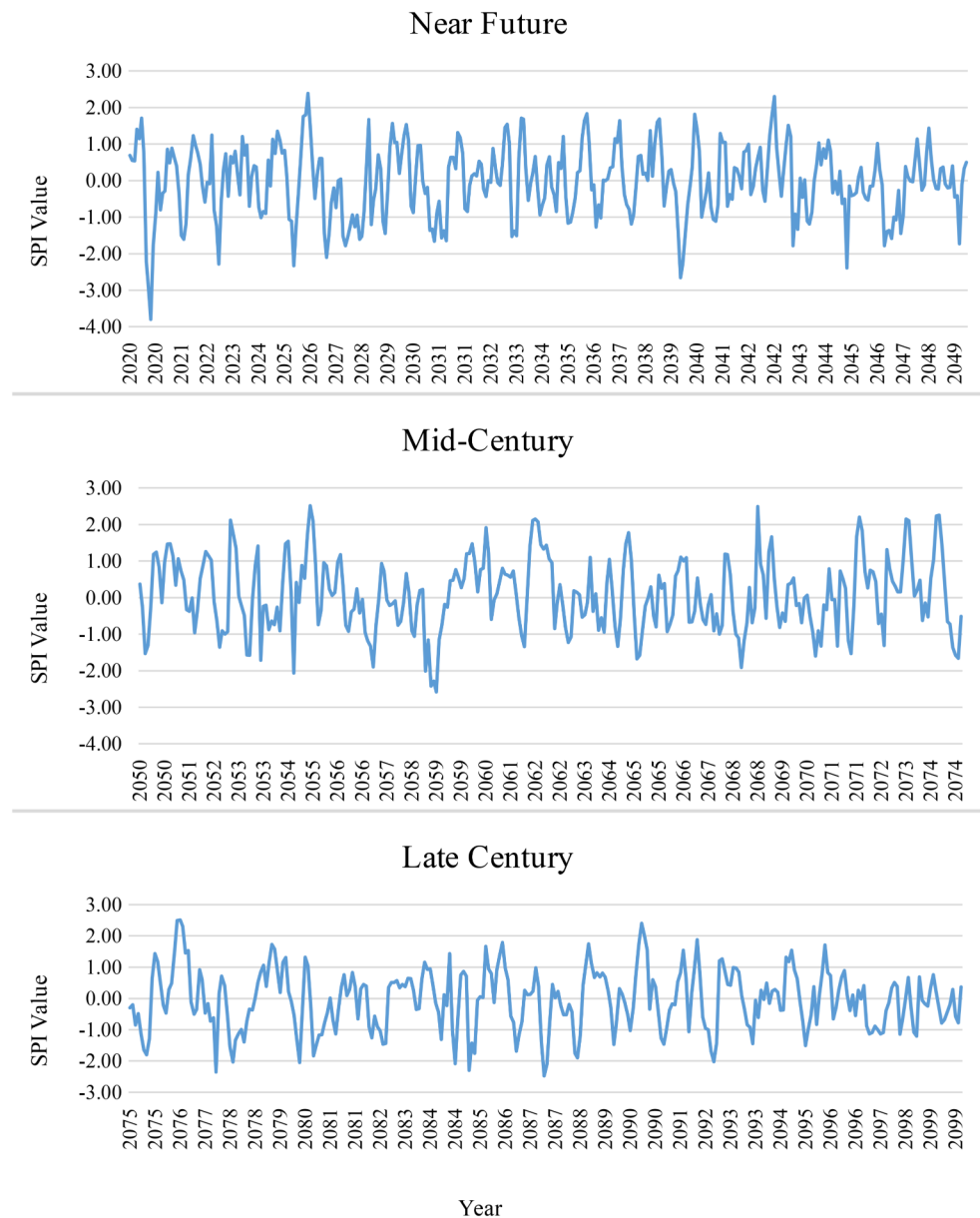
Fig. 2 SPI-3 index time series according to SSP2-4.5 scenario
