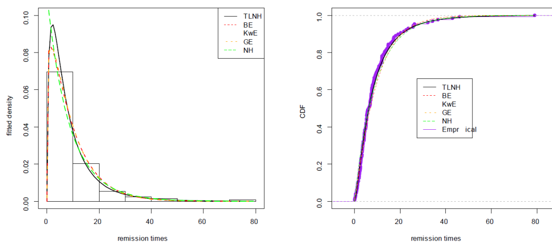
Figure 2. The estimated pdfs (left) and cdfs (right) for the remission data.
